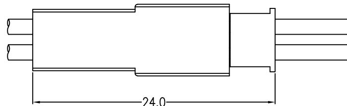
Assembly Layout
